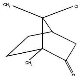
Figure 1: Molecular structure of camphor.
